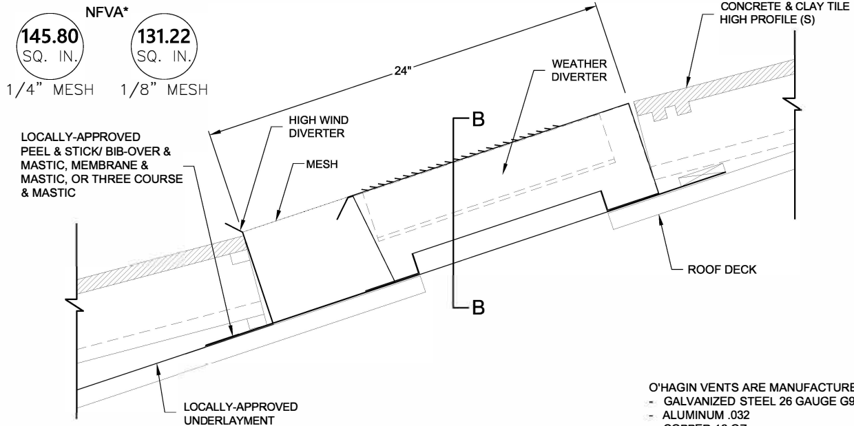
ELEVATIONS
